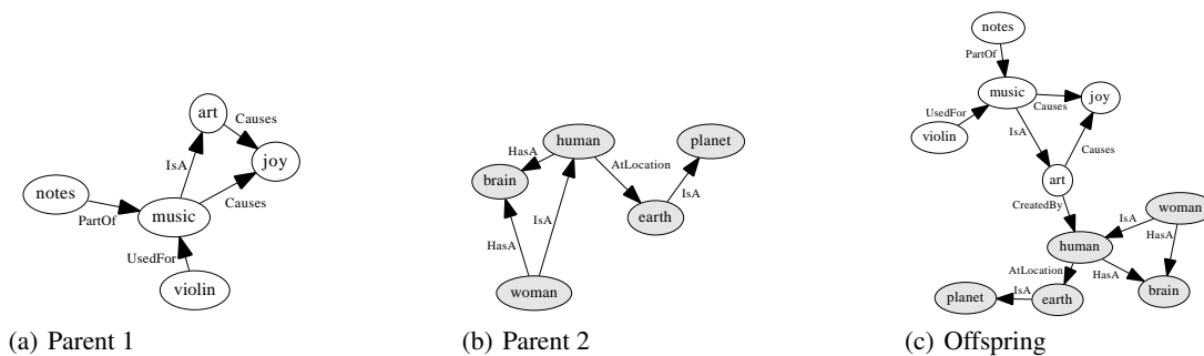
Figure 2: Commonsense crossover type II (graph merging crossover), merging by the relation CreatedBy(art, human) . If no concepts attachable through commonsense relations are encountered, the offspring is formed by merging the parent networks as two separate clusters within the same semantic network.
